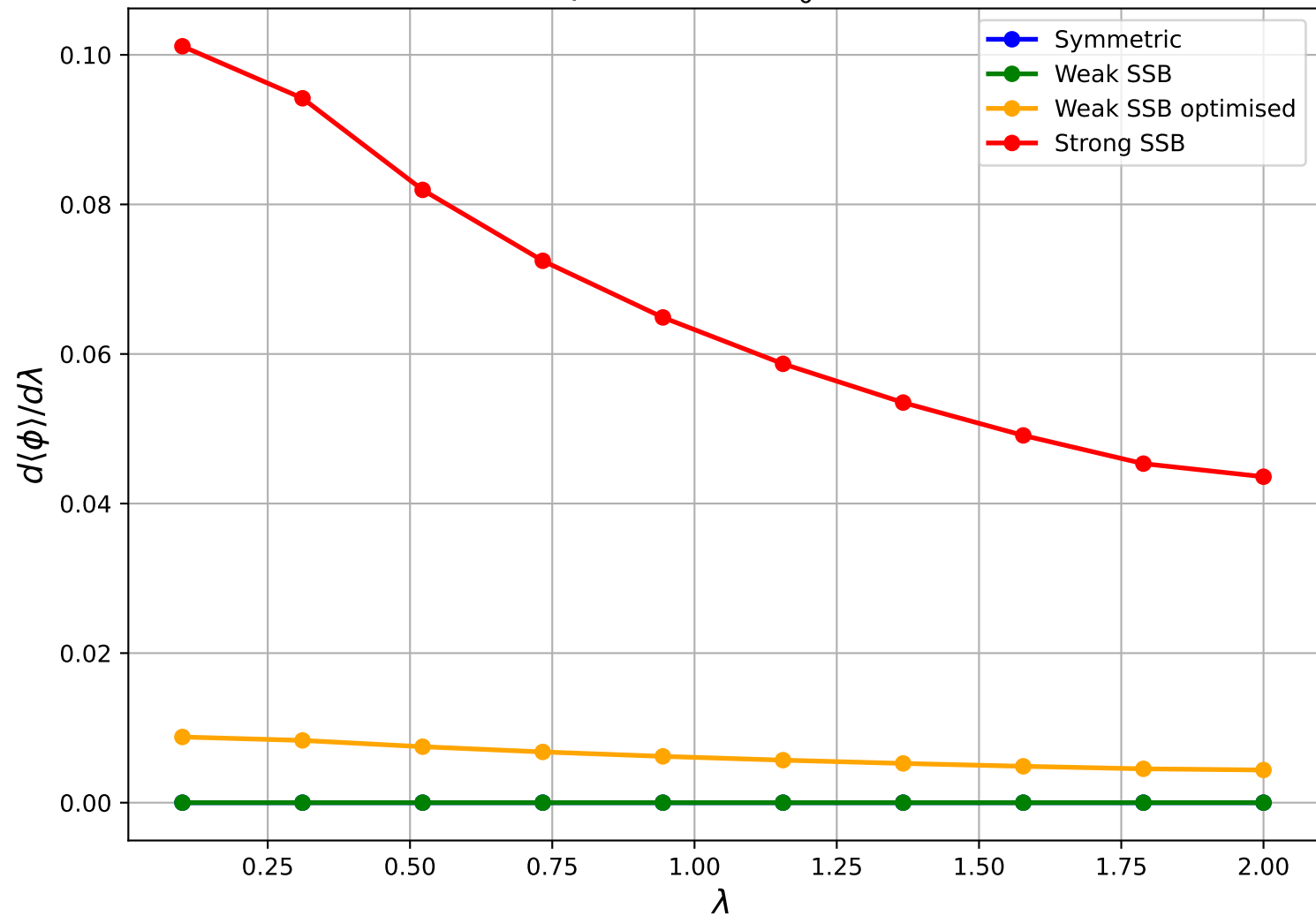
d\langle\phi\rangle/d\lambda vs \lambda , m_0^2 = 1.0
